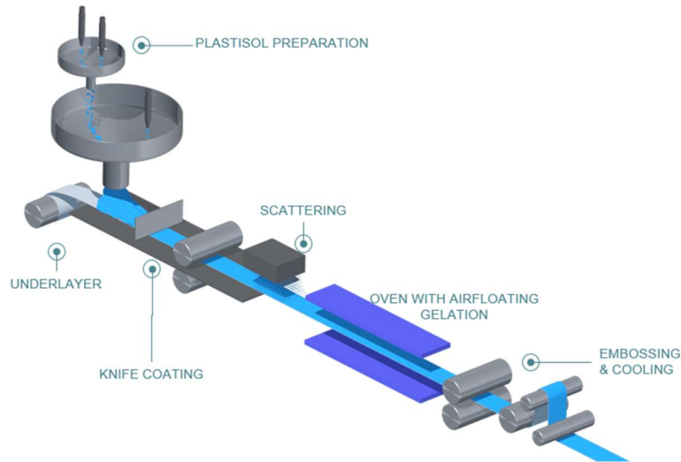
Process flow diagram (coating)
